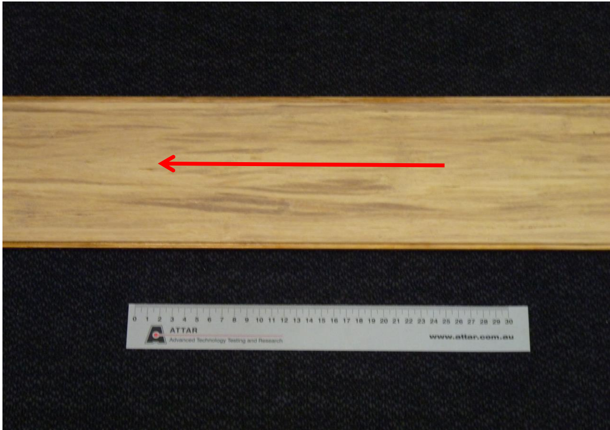
Figure 1: Strand Woven Bamboo 14mm timber flooring Arrow indicates direction of testing
